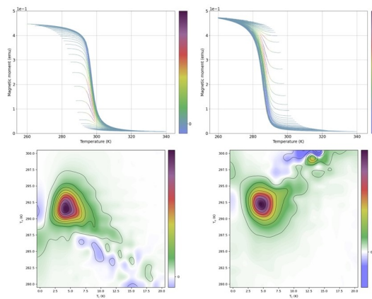
Figure 1: TFORCs in heating and cooling modes of (\text{NiMnSi})_{0.66}(\text{Fe}_2\text{Ge})_{0.34} and corresponding TFORC distributions
